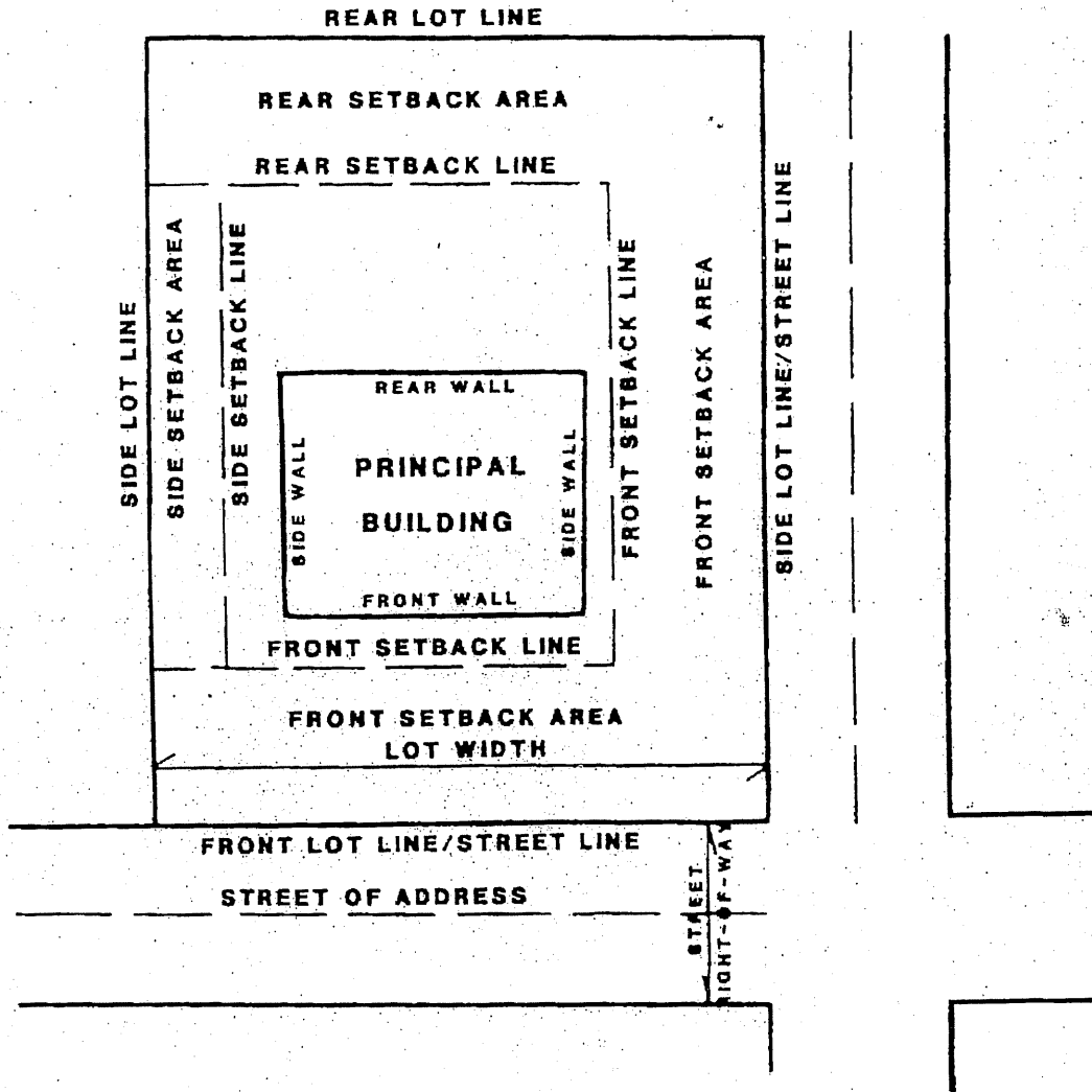
ILLUSTRATION DEPICTING SETBACK REQUIREMENTS APPLYING TO CORNER LOTS
